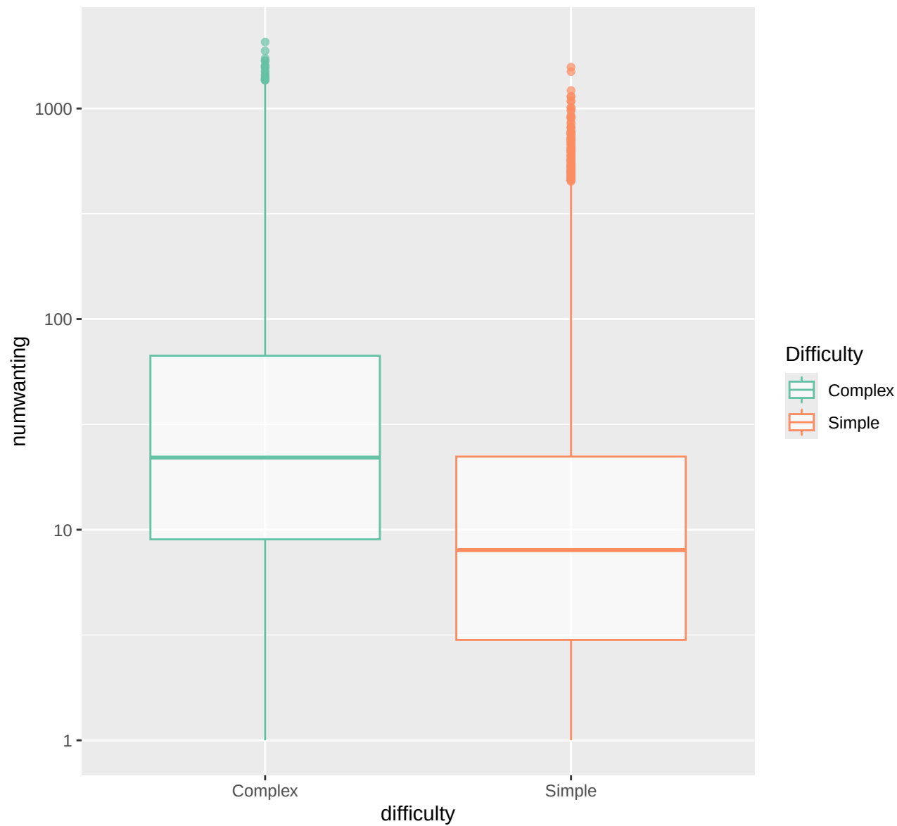
Log NumWanted by Difficulty
